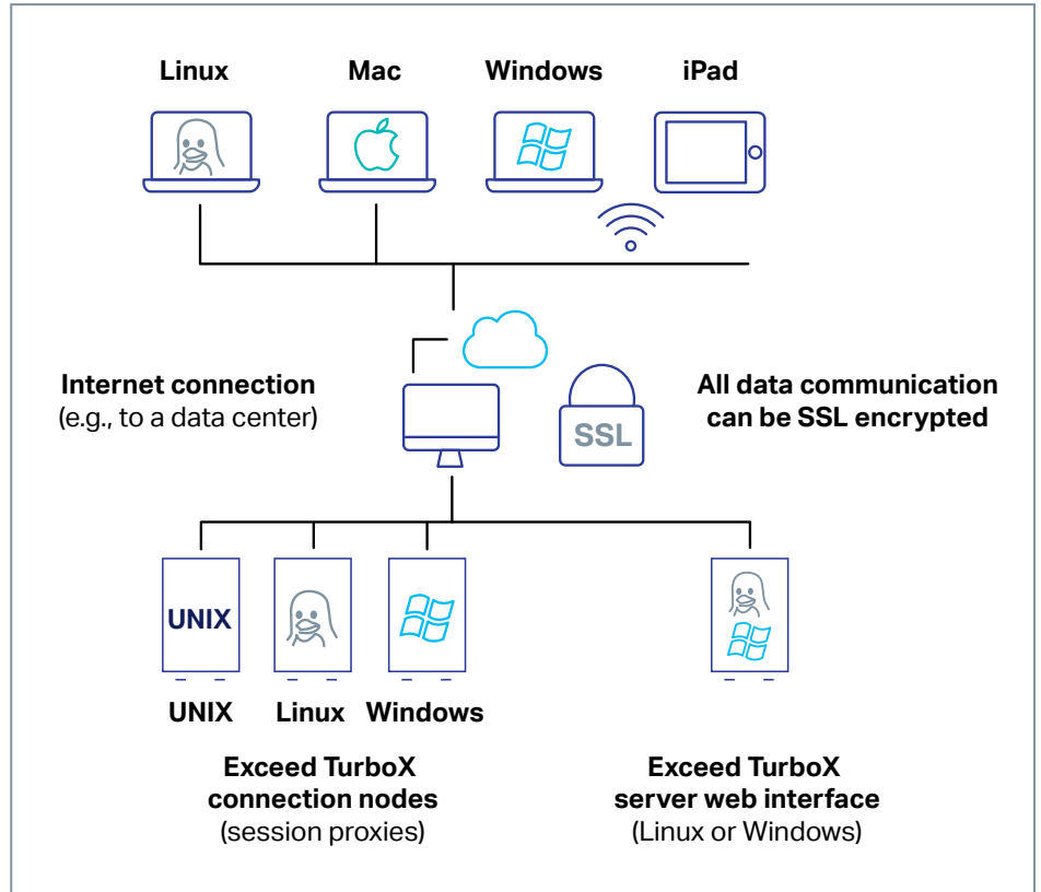
OpenText Exceed TurboX Architecture
